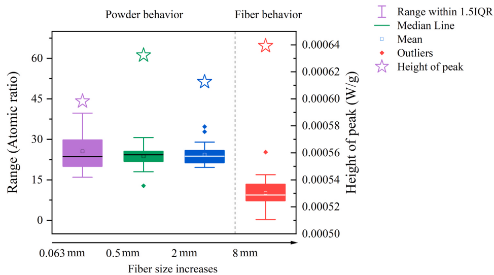
Fig. 20. Effect of WTB waste fiber size on cement hydration.
