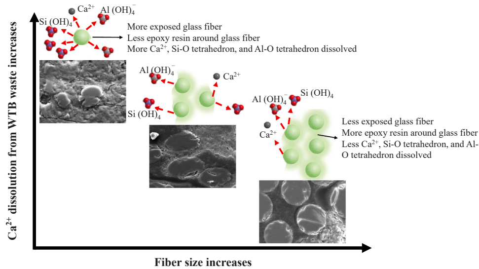
Fig. 19. Effect of fiber size on the dissolution of WTB waste.
