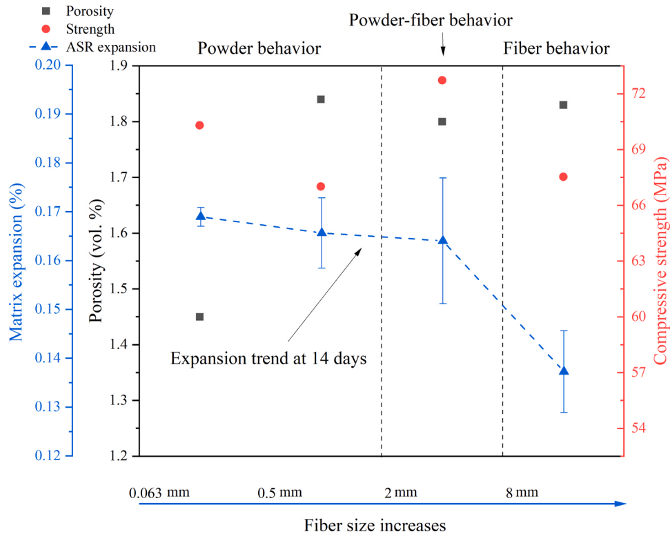
Fig. 21. Effect of WTB waste fiber size on strength and ASR.
