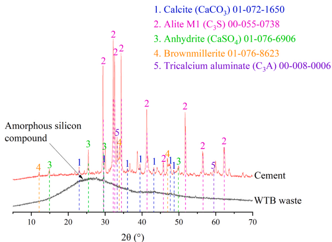
Fig. 2. XRD diffractograms of WTB waste (black) and unhydrated cement (red line).
