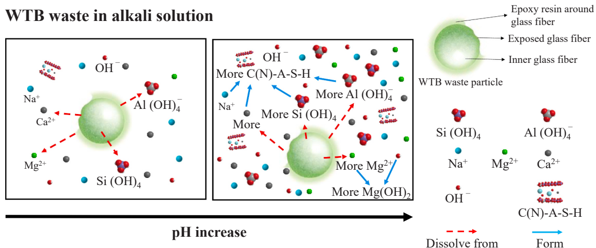
Fig. 18. Effect of pH on the dissolution of WTB waste and precipitation.
